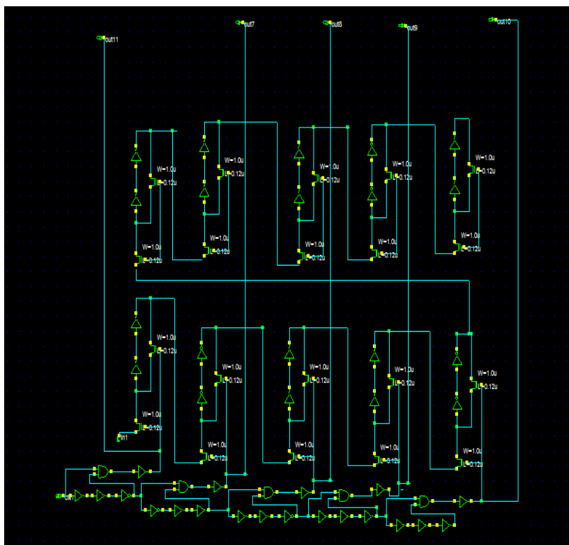
Fig.6: Proposed shift register
