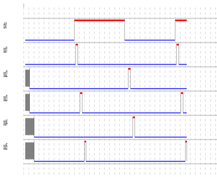
Fig.7: Simulation Waveform
