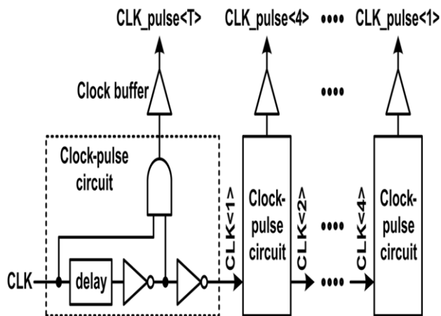
Fig.5: Delayed pulsed clock generator.
