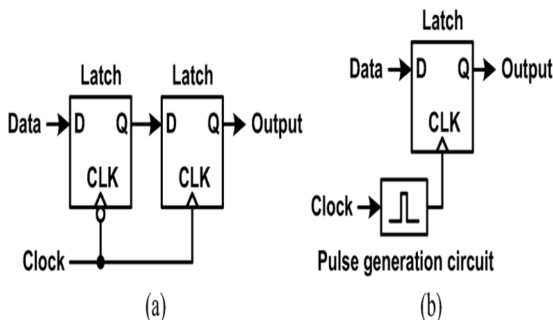
Fig.1: (a) Master-slave flip-flop. (b) Pulsed latch.
